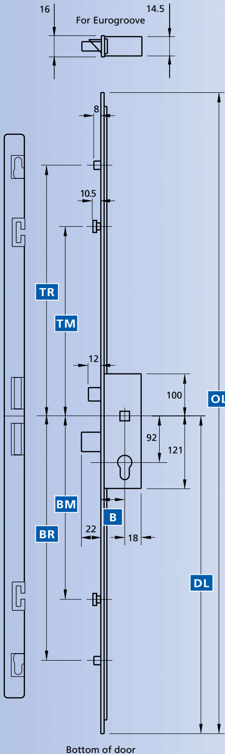
Diagram illustrates product in locked position. Not to scale.
